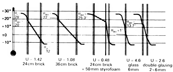
⑦ Temperature variation across variously insulated components for an internal temperature \theta_i = 28^\circ and outside air temperature \theta_a = -12^\circ
